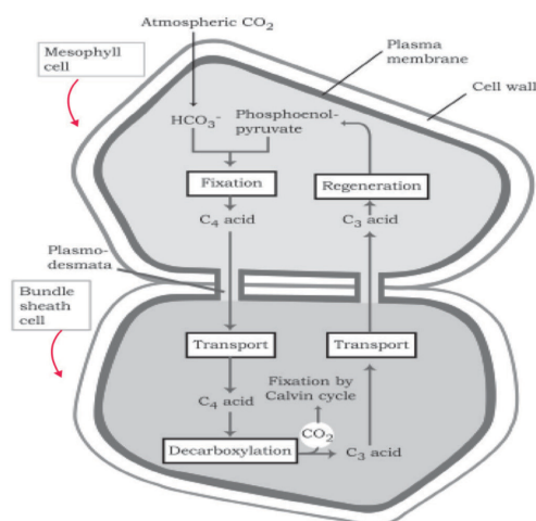
Figure 13.9 diagrammatic representation of the Hatch and Slack Pathway
