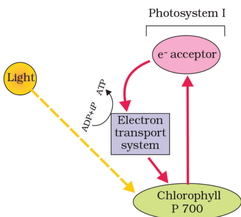
Figure 13.6 Cyclic photophosphorylation
