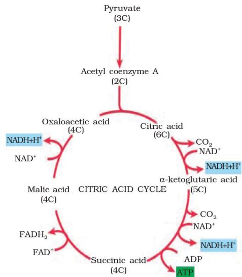
Figure 14.3 The Citric acid cycle
